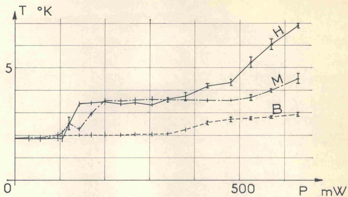
FIG. 5 : Superfluid helium T = 1.85 K; P = 335 mm Hg
