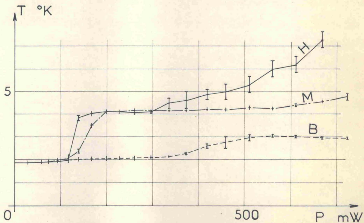
FIG.6 : Superfluid helium T = 1.85 K ; p = 1 atm
